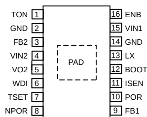
Pin-out Diagram
