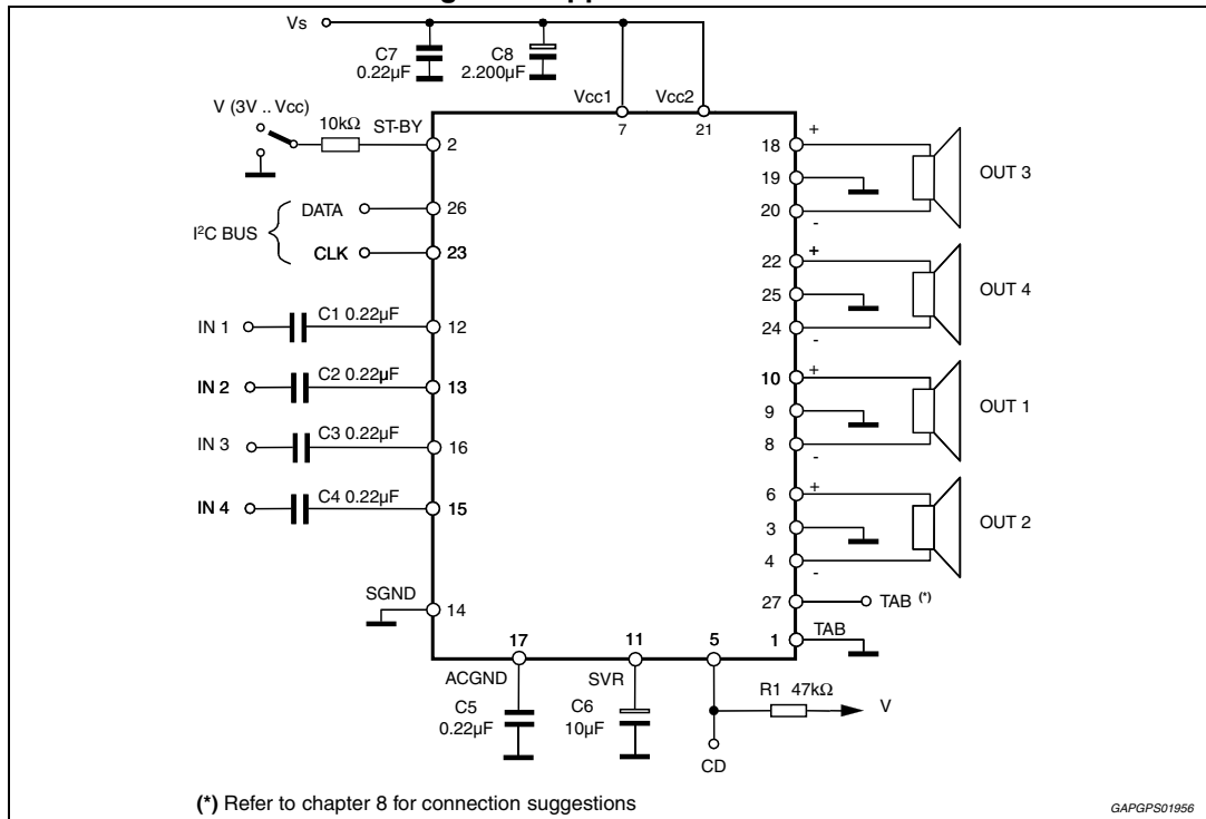
Figure 2. Application circuit
