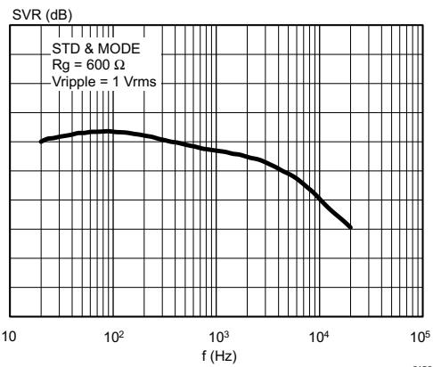
Figure 15. Supply voltage rejection vs. frequency
