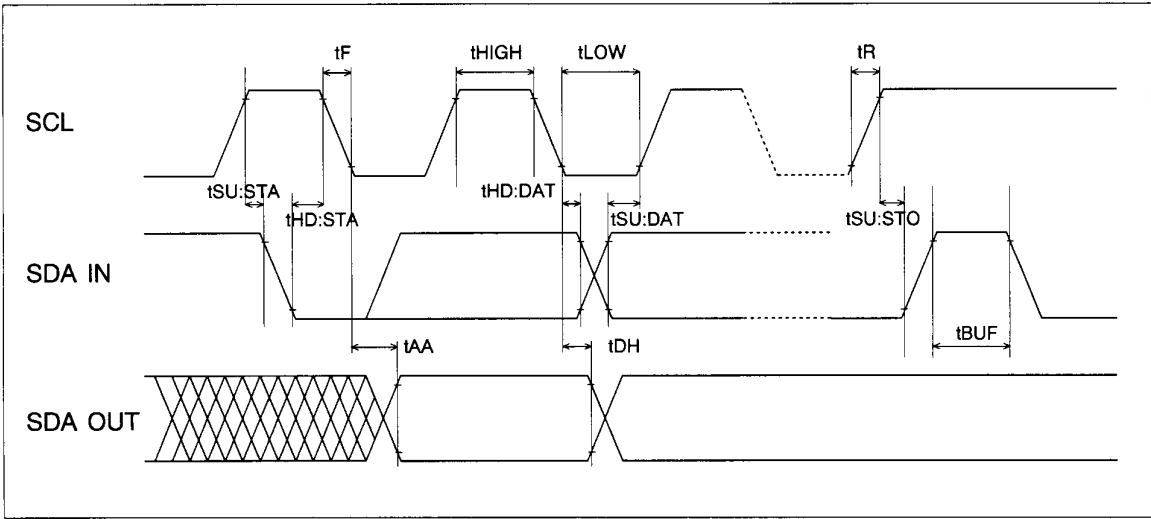
BUS TIMING
