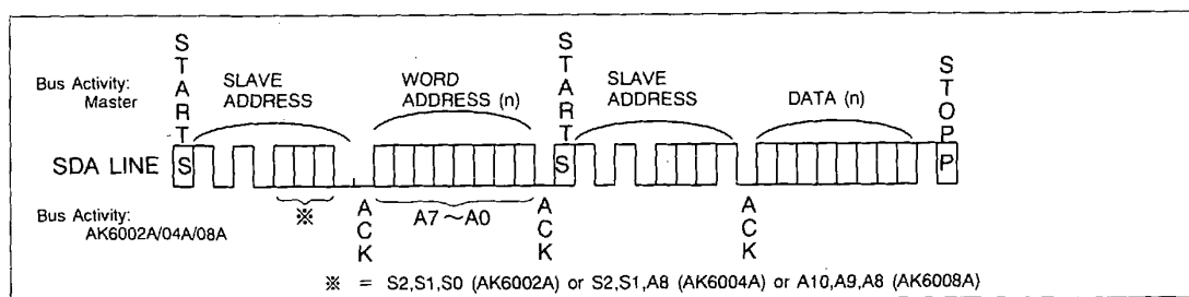
RANDOM READ
