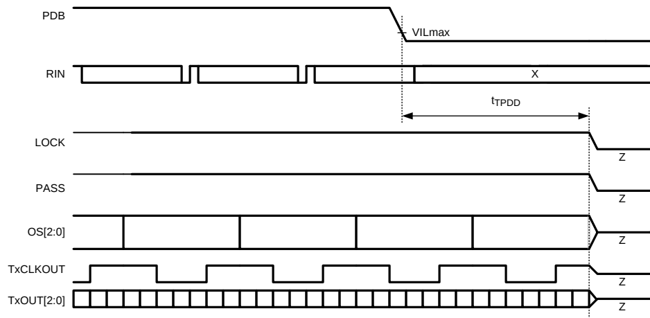
Figure 6. FPD-Link &amp; LVCMOS Powerdown Delay
