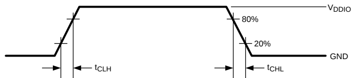
Figure 5. LVCMOS Transition Times
