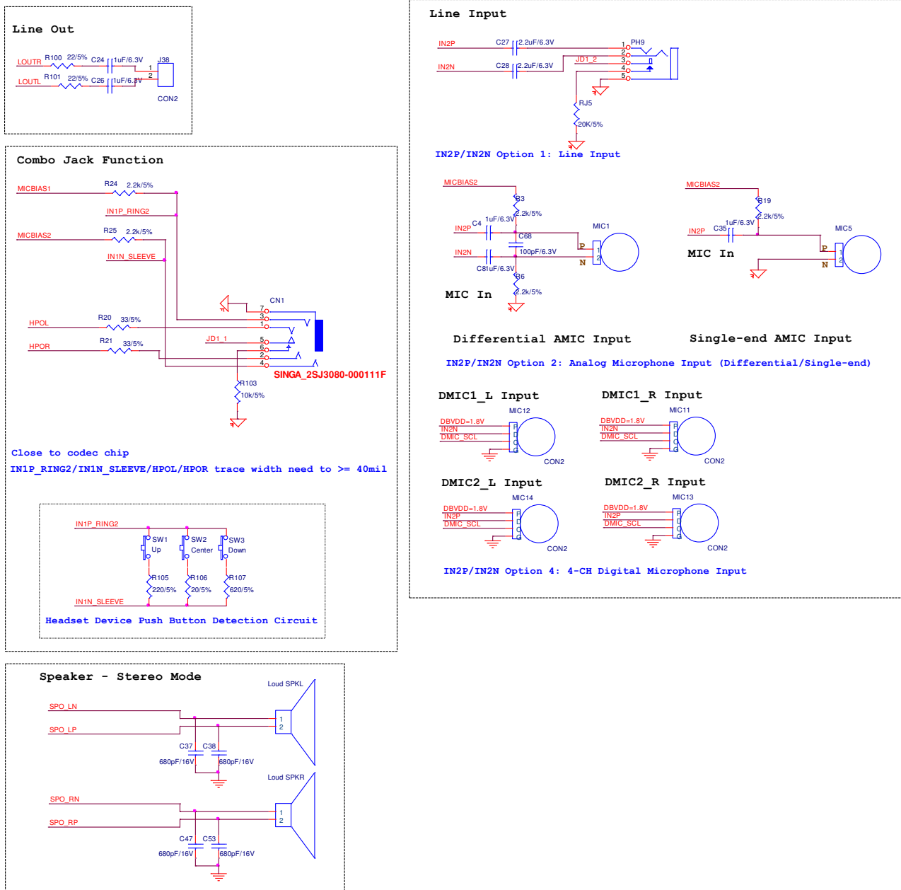
Figure 36. Application Circuit
