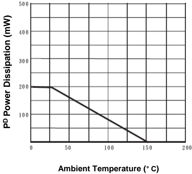
Fig.1- Forward Power Dissipation Derating Curve
