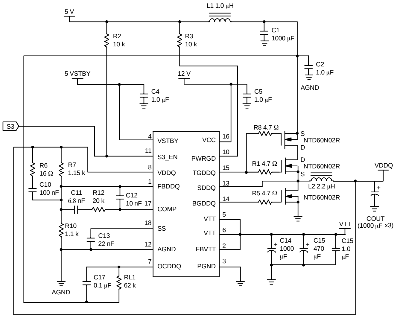
Figure 1. Application Diagram
