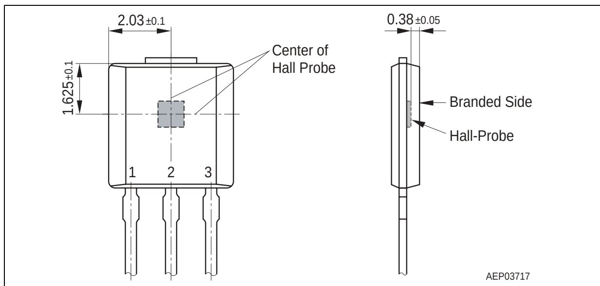
Figure 1 TLE4998P3 Pin Configuration and Hall Cell Location
