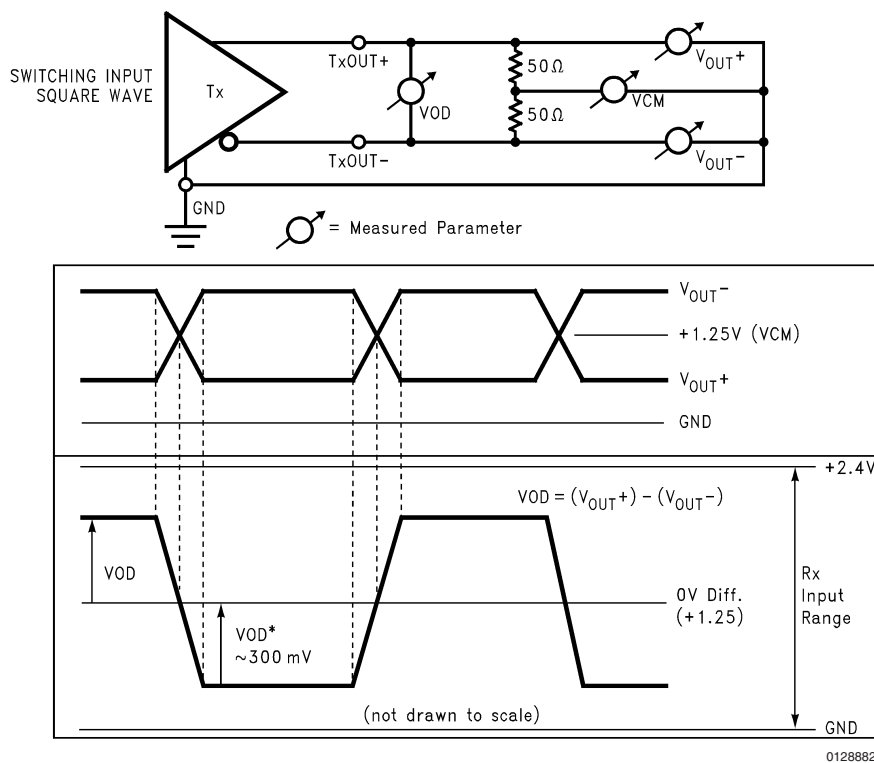
FIGURE 20. Single-Ended and Differential Waveforms
