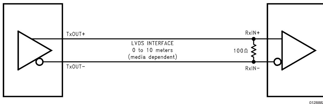
FIGURE 18. LVDS Serialized Link Termination
