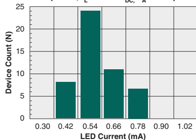
Typical I_F for Switch Operation (N=50, I_L=120\text{mA}_{\text{DC}} , T_A=25^\circ\text{C} )
