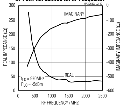
MAX2680 RF PORT IMPEDANCE vs. RF FREQUENCY
