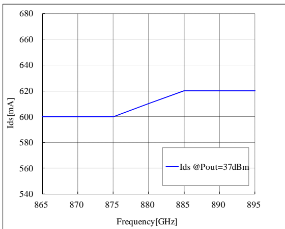
Total Ids vs. Frequency
