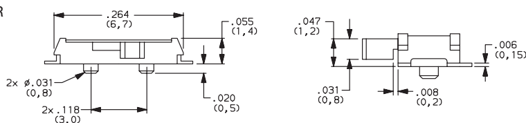
PCM12SMTR SPDT
