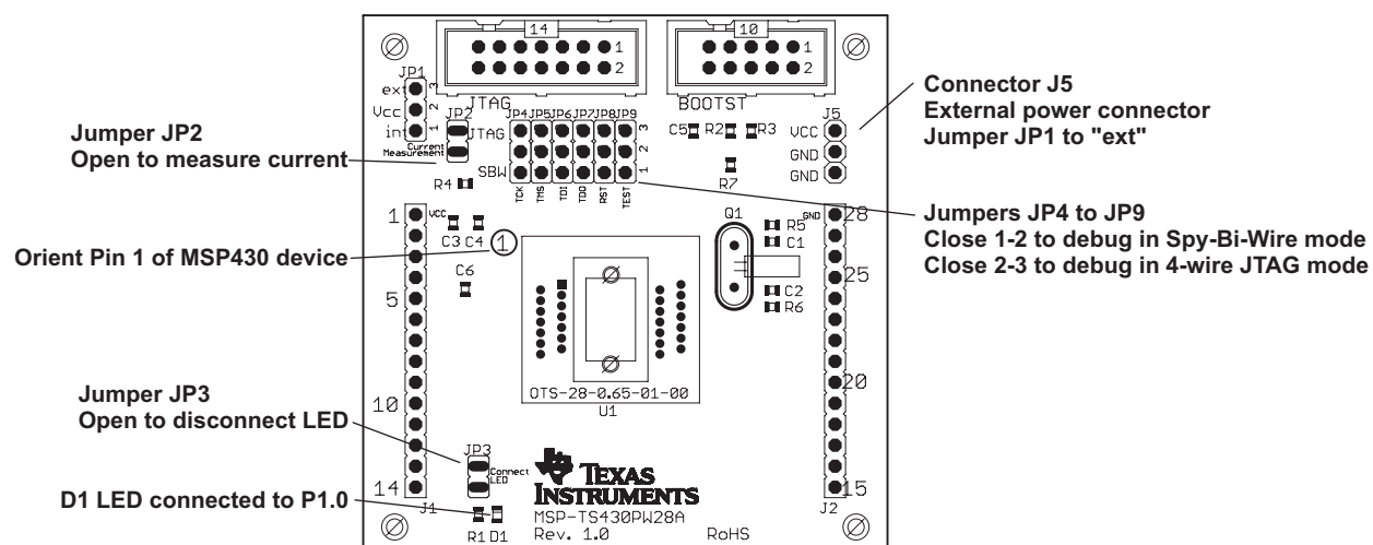
Figure B-14. MSP-TS430PW28A Target Socket Module, PCB (Red)
