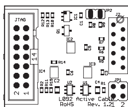
Figure B-6. MSP-TS430L092 Active Cable Target Socket Module, PCB
