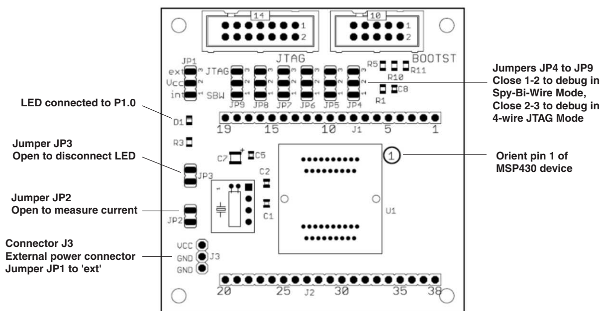
Figure B-16. MSP-TS430DA38 Target Socket Module, PCB
