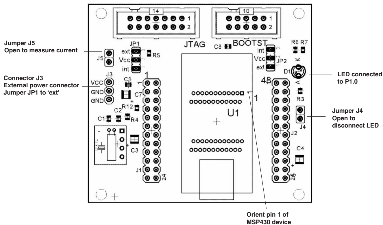
Figure B-24. MSP-TS430DL48 Target Socket Module, PCB
