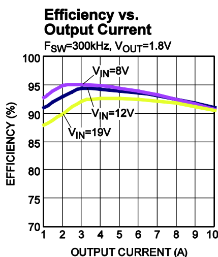
Figure 35 — Efficiency Curve
