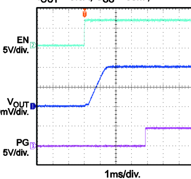
Power Good through EN Start Up I_{OUT} = 0.5A , C_{SS} = 33nF ,
