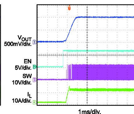
Start up through EN I_{OUT} = 10A
