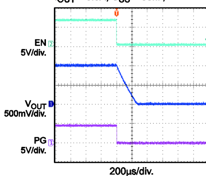
Power Good through EN Shutdown I_{OUT} = 0.5A , C_{SS} = 33nF ,
