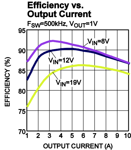
Figure 13 — Efficiency Curve MPQ8636-10, MPQ8636H-10, V_{OUT}=1V , I_{OUT}=1A-10A , f_{SW}=500kHz
