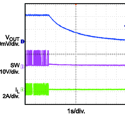
Thermal Shutdown I_{OUT} = 0A
