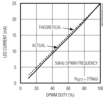
LED CURRENT vs. DPWM DUTY
