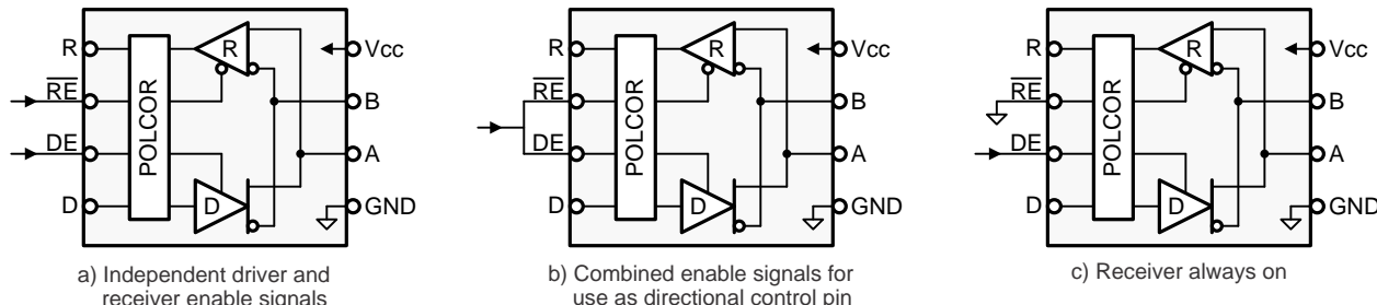
Figure 13. Transceiver Configurations
