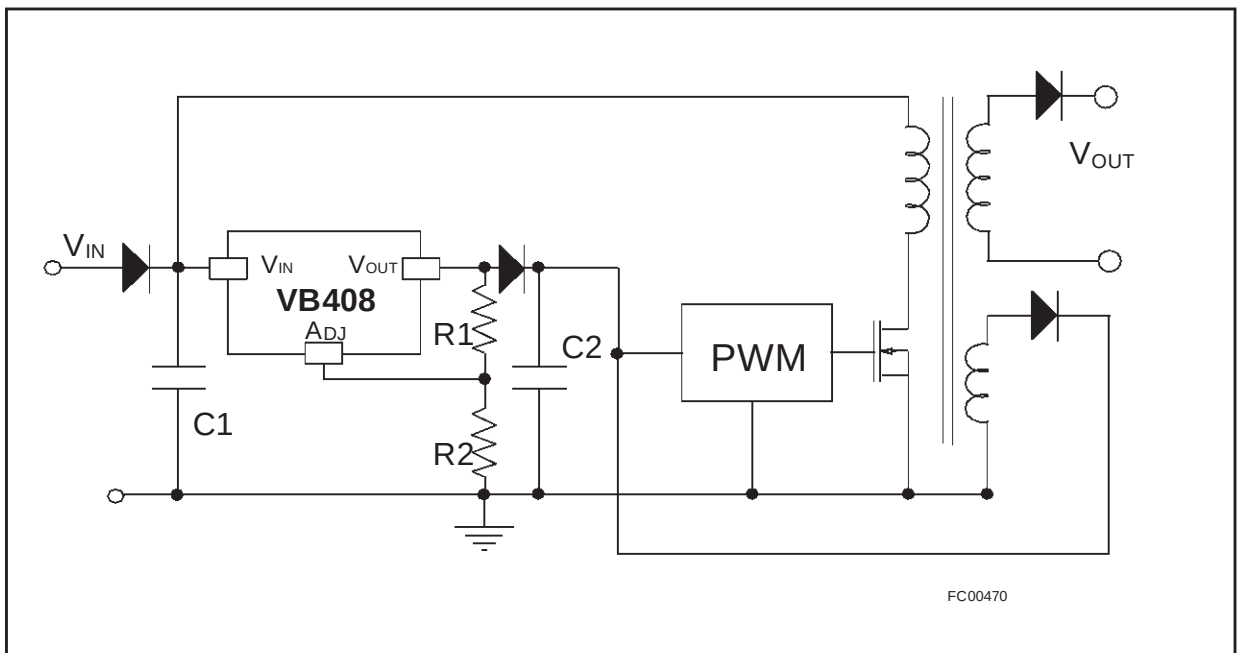
Figure 3: Start-up circuit
