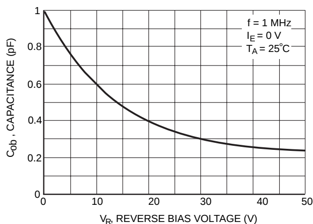
Figure 14. Output Capacitance
