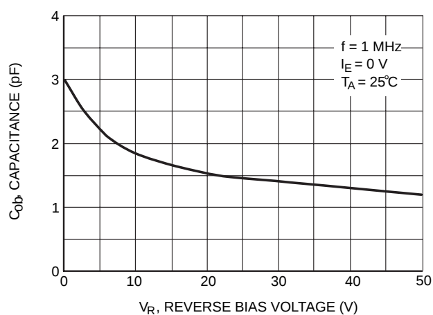
Figure.9 Output Capacitance
