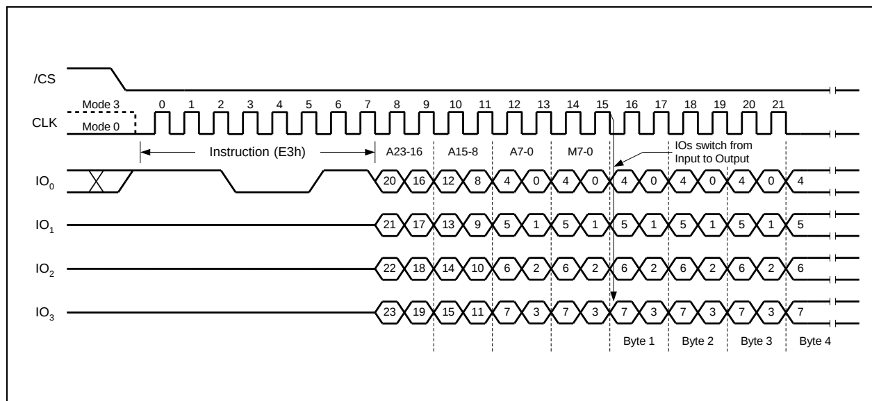
Figure 16a. Octal Word Read Quad I/O Instruction Sequence (Initial instruction or previous M5-4 ≠ 10)
