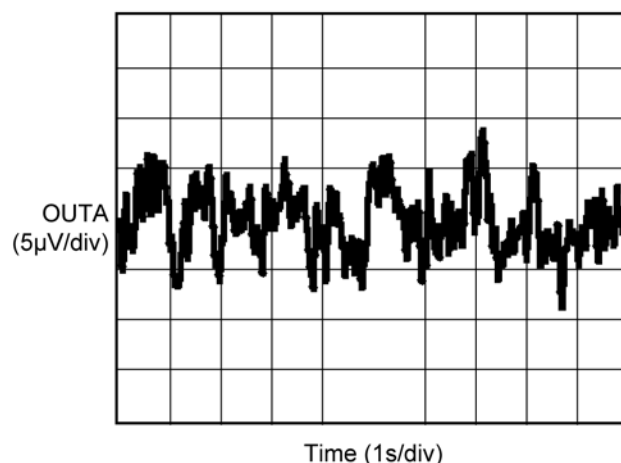
0.1Hz to 10Hz Input Referred Voltage Noise
