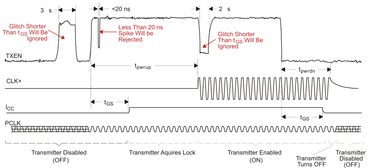
Figure 15. Transmitter Enable Glitch Suppression Time
