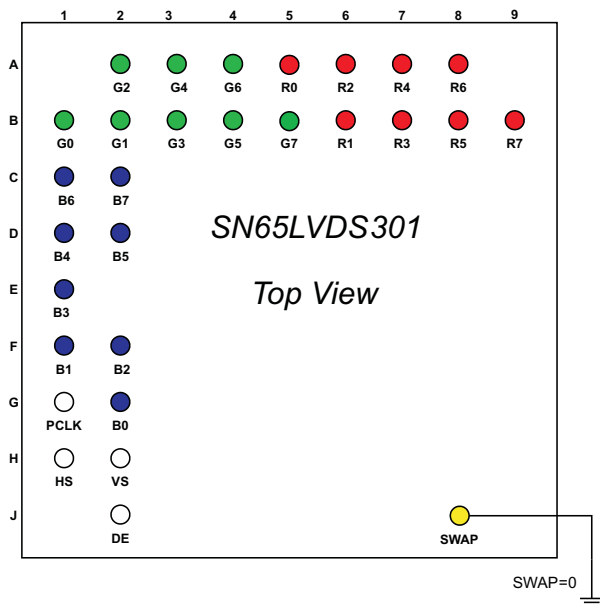
Figure 1. SWAP PIN = 0
