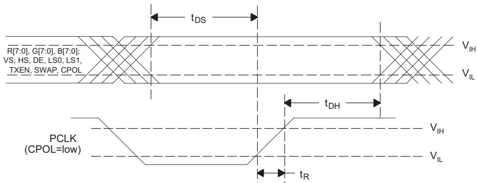
Figure 8. Setup/Hold Time
