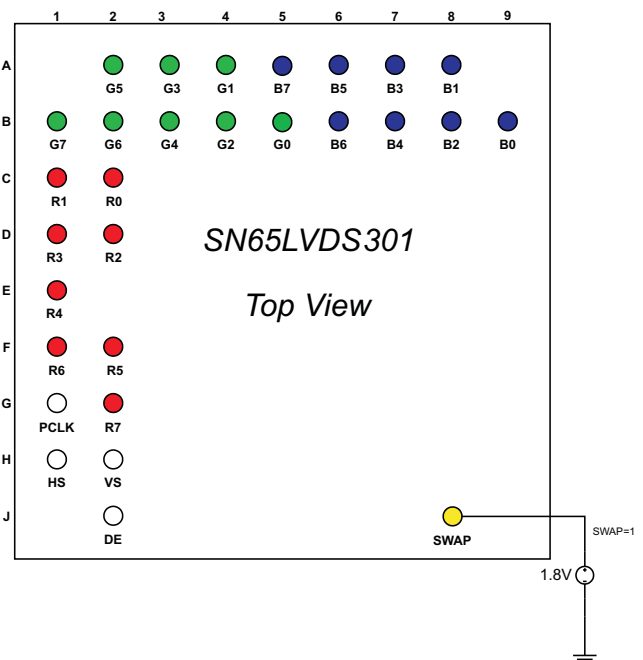
Figure 2. SWAP PIN = 1
