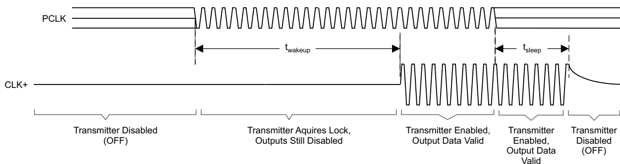
Figure 16. Standby Detection
