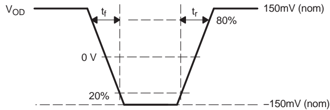
Figure 9. Rise and Fall Time Definitions
