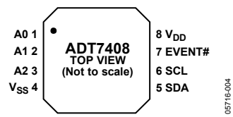
Figure 4. Pin Configuration
