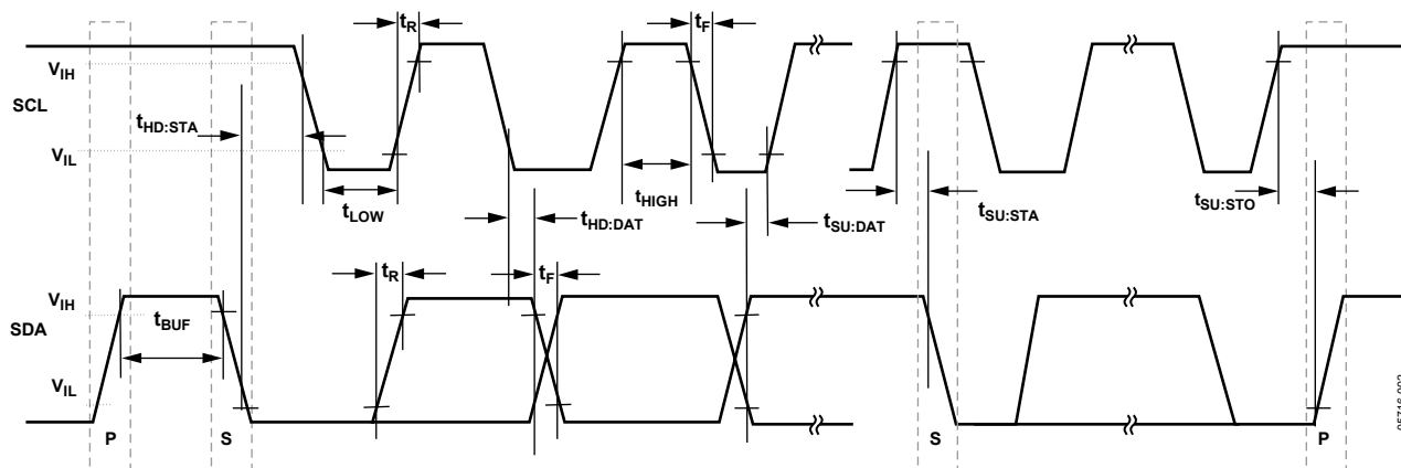
Figure 2. SMBus/I²C Timing Diagram
