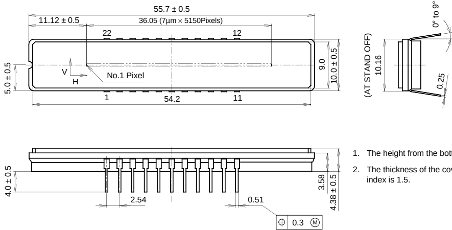
22pin DIP (400mil)
