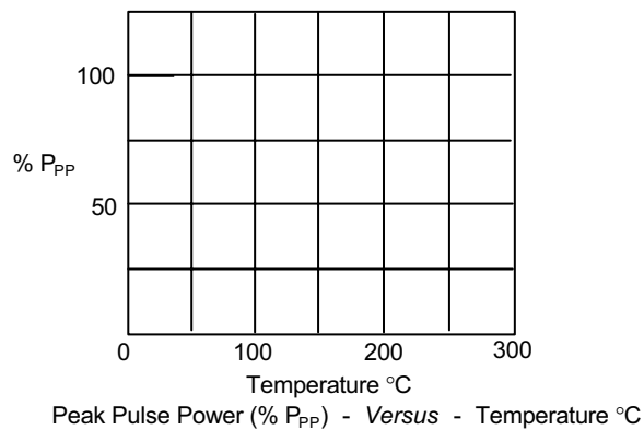
Figure 4 - Derating Curve
