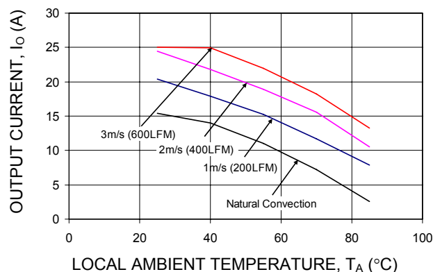
Figure 14. Output Current Derating for the QBE025A0B in the Transverse Orientation with no baseplate; Airflow Direction from V_{in}(+) to V_{in}(-) ; V_{in} = 48 V
