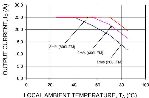
Figure 17. Output Current Derating for the QBE025A0B ( V_o = 12V ) in the Transverse Orientation with baseplate and 0.5-inch high heatsink; Airflow Direction from Vin(–) to Vout(–); Vin = 48V
