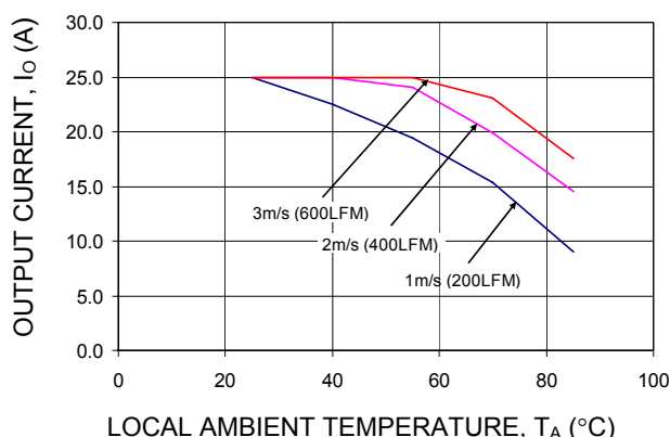
Figure 16. Output Current Derating for the QBE025A0B ( V_o = 12V ) in the Transverse Orientation with baseplate and 0.25-inch high heatsink; Airflow Direction from Vin(–) to Vout(–); Vin = 48V
