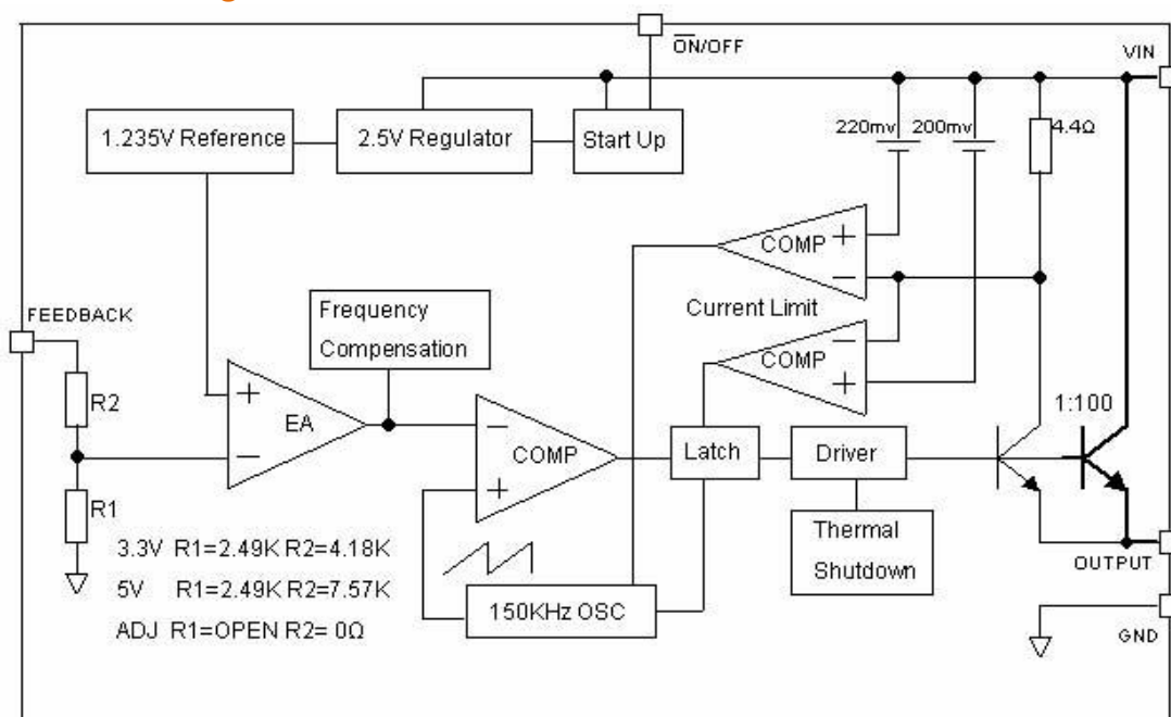
Figure 3 Function Block Diagram of EC9301A
