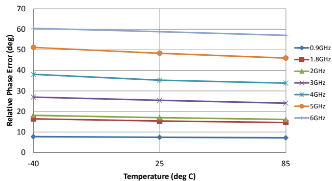
Figure 25. Relative Phase Error for 31.75 dB Attenuation Setting vs. Frequency
