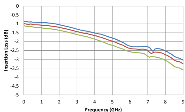
Figure 19. Insertion Loss vs. Temperature
