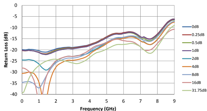
Figure 21. Output Return Loss vs. Attenuation Setting
