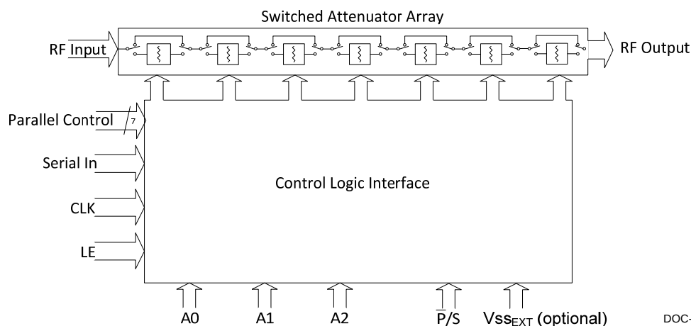
Figure 2. Functional Diagram
