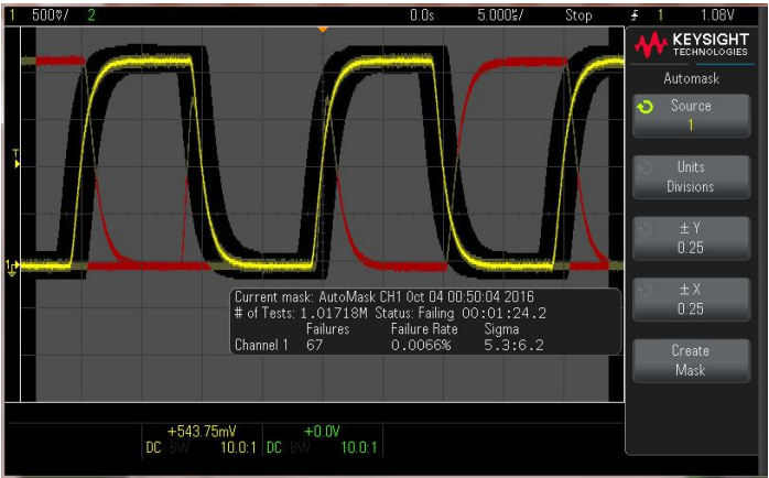
Mask testing can quickly validate signal quality and detect errors.
