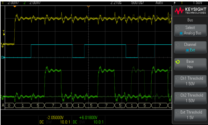
Channel 1, 2 and external trigger can be combined to form a bus with hex or binary values displayed as the bus along the bottom of the display.
