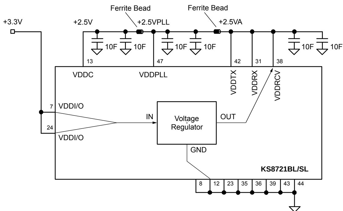
Figure 4. Circuit Design
