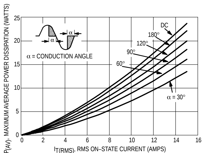
Figure 2.0 Maximum On-State Power Dissipation
