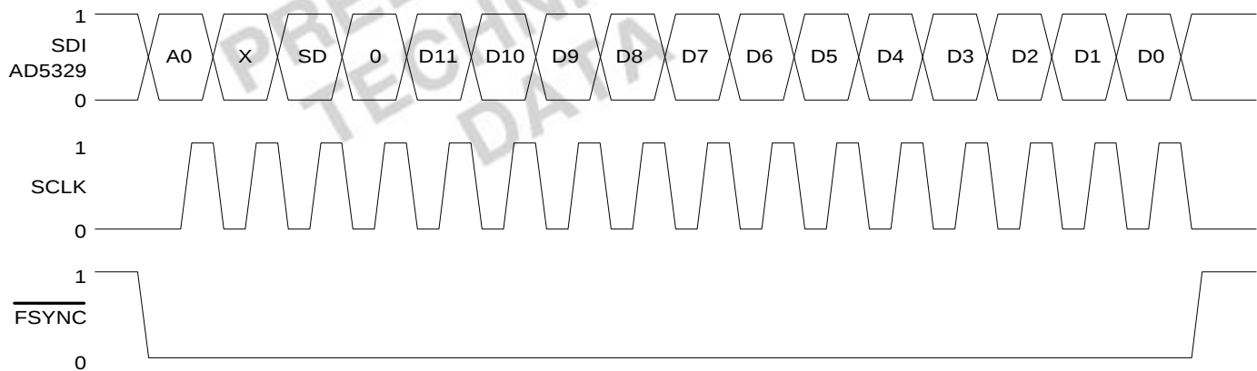
Figure 1A. Timing Diagram
