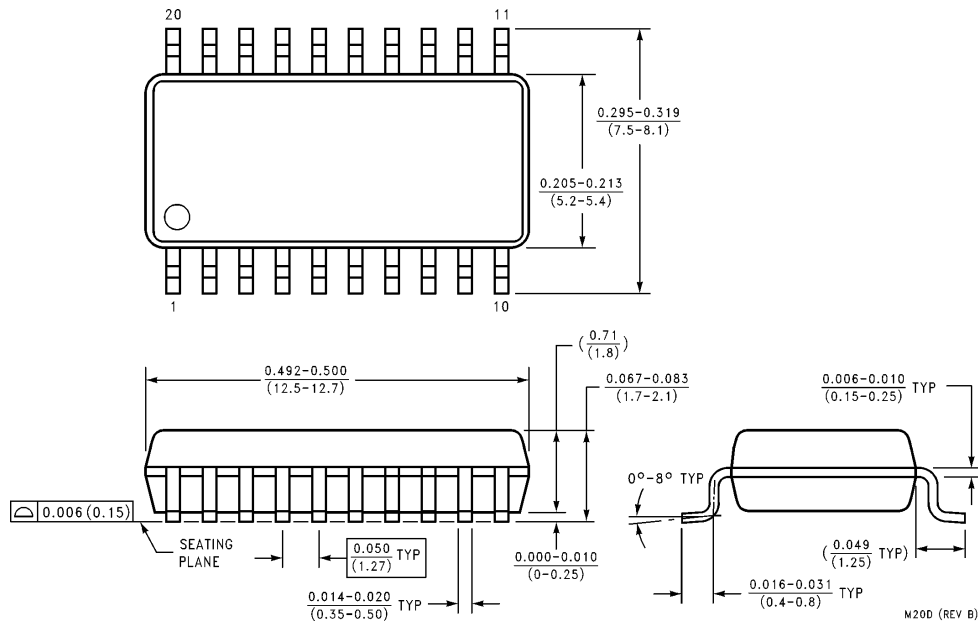
20-Lead Small Outline Package EIAJ SOIC (SJ) Order Number 74LVX373SJ or 74LVX373SJX NS Package Number M20D
