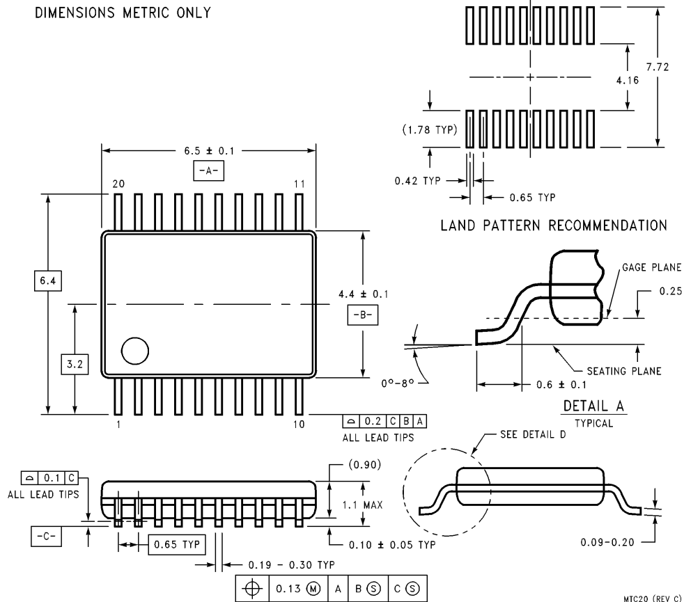
16-Lead Thin Shrink Small Outline Package, JEDEC Order Number 74LVX373MTC or 74LVX373MTCX NS Package Number MTC20
