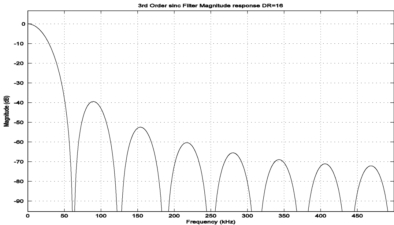
Figure 15. Sinc Filter Response, t s = 16 μs
