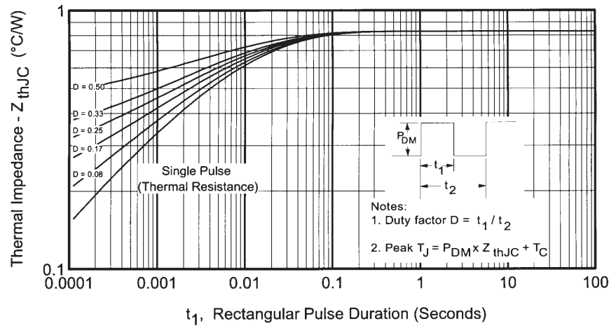
Fig. 4 - Max. Thermal Impedance Z_{thJC} Characteristics (Per Leg)
