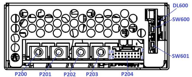
Figure 9. Rear View - MBE1200-1T24 / MBE1200-1T48 Models
