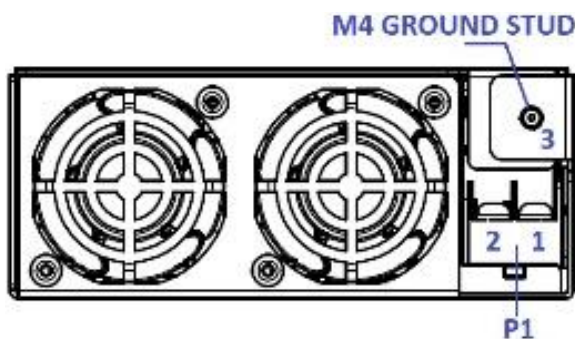
Figure 8. Front View - MBE1200-1T24 / MBE1200-1T48 Models
