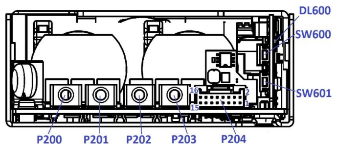
Figure 6. Rear View - MBC1200-1T24-UCF Model
