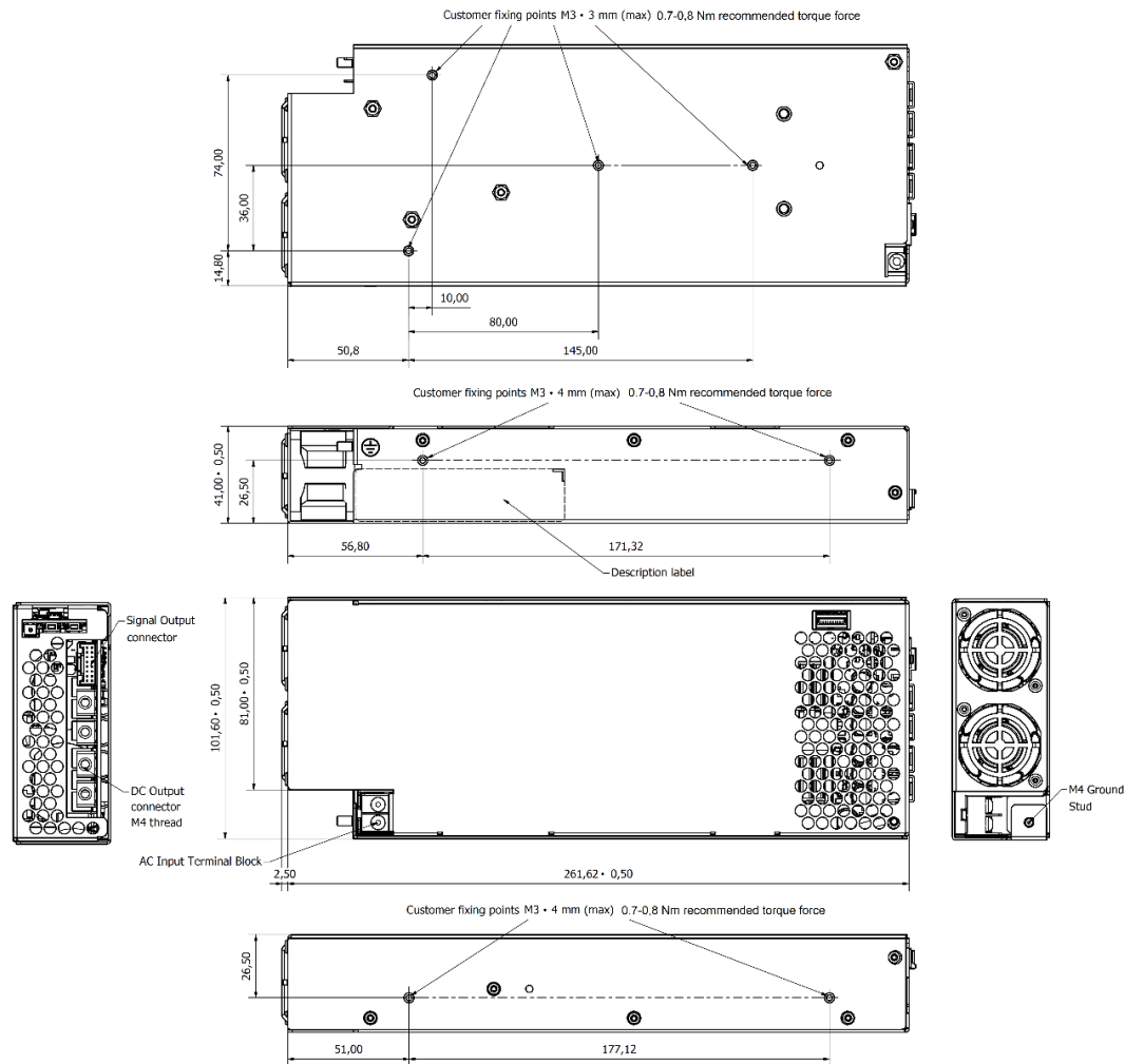
Figure 7. Mechanical Drawing - MBE1200-1T24 / MBE1200-1T48 Models
