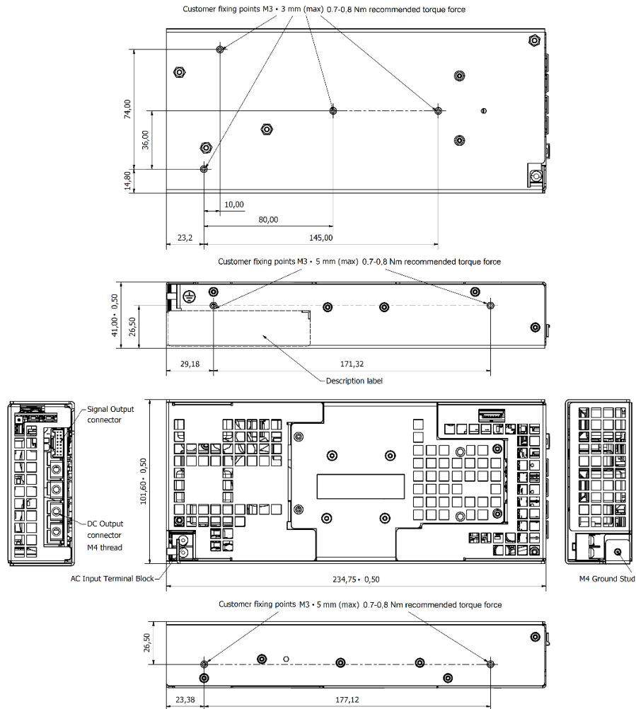
Figure 4. Mechanical Drawing - MBC1200-1T24-PCF Model
