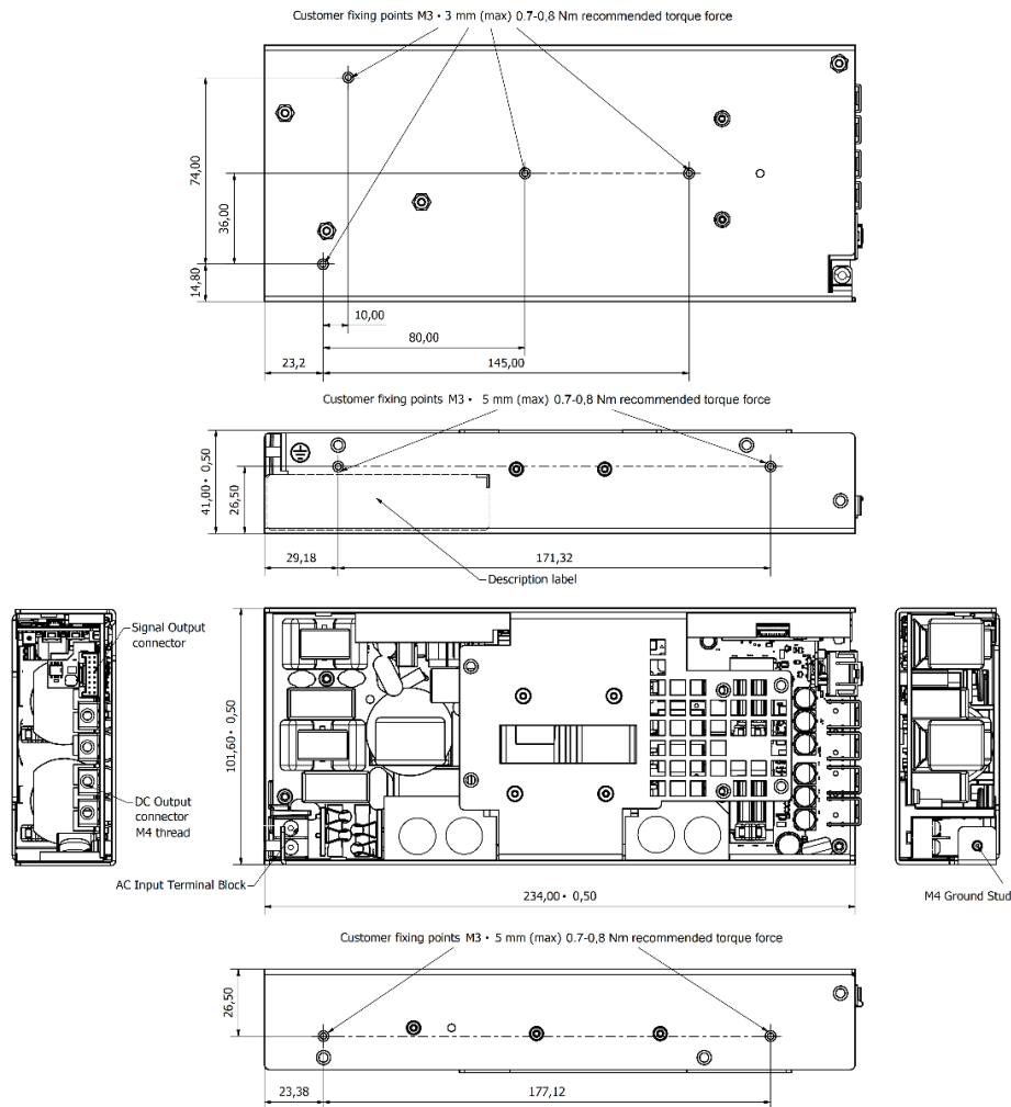
Figure 1. Mechanical Drawing - MBC1200-1T24-UCF Model
