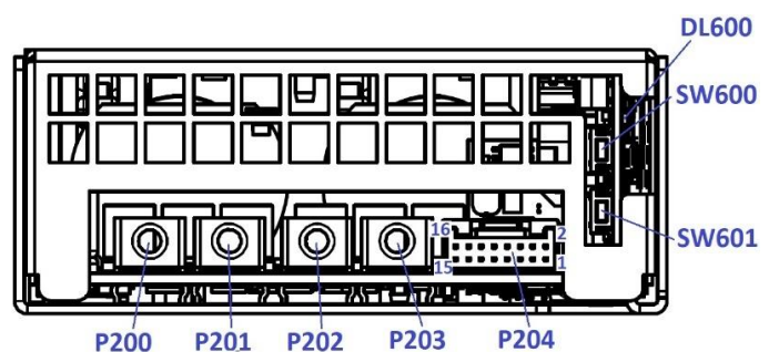
Figure 6. Rear View - MBC1200-1T24-PCF Model
