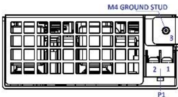
Figure 5. Front View - MBC1200-1T24-PCF Model
