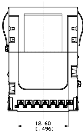
VIEW T
