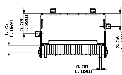
VIEW S
