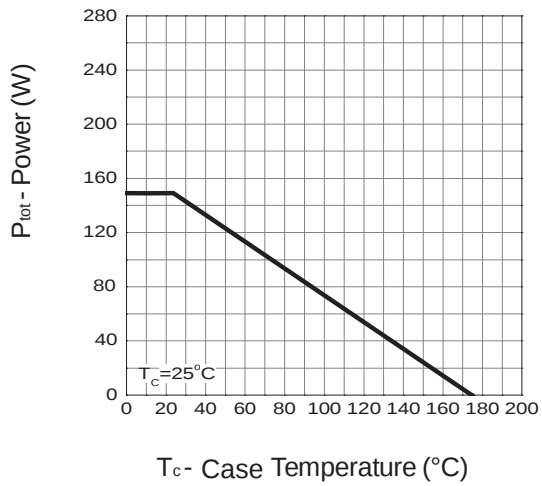
Power Dissipation
