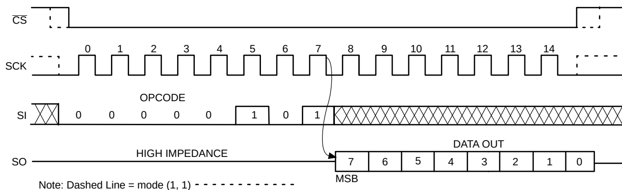
Figure 10. RDSR Timing
