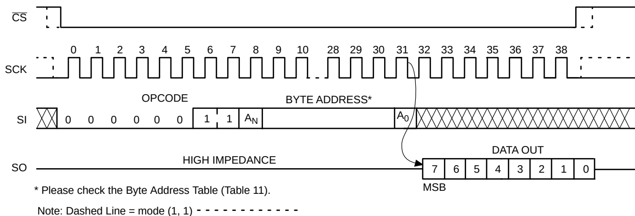
Figure 9. READ Timing
