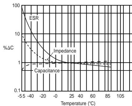
Temperature Characteristics - 29,000 \mu\text{F} 50 Vdc
