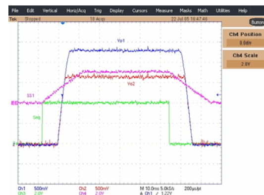
Fig. 14: Simultaneously Power Up / down
