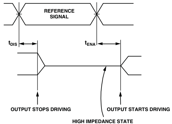
Figure 62. Output Enable/Disable
