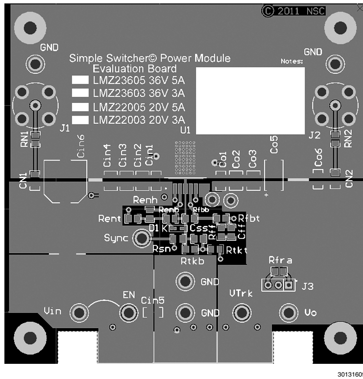
FIGURE 3. Top Layer
