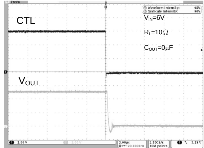
Fig. 13 Turn-Off Time
