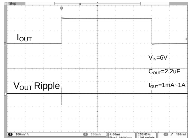
Fig. 17 Load Transition
