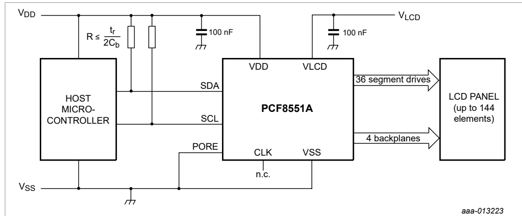
Figure 8. Typical system configuration using I²C-bus, internal power-on reset disabled
