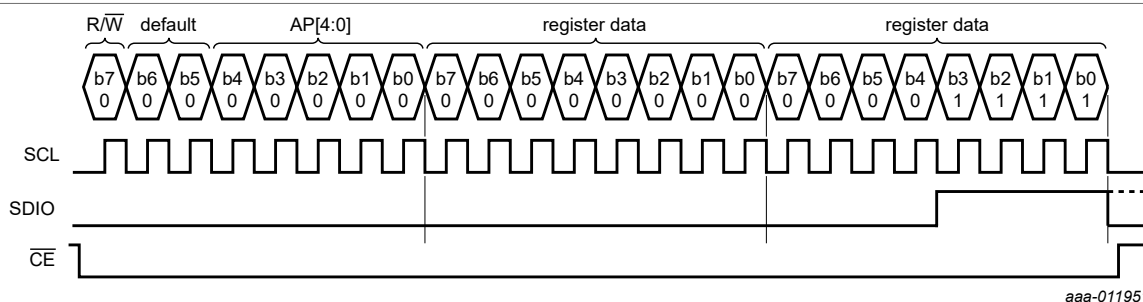
Figure 20. SPI-bus write example: writing two data bytes to registers 00h and 01h
