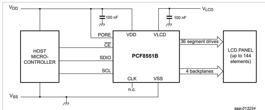
Figure 9. Typical system configuration using SPI-bus, internal power-on reset enabled
