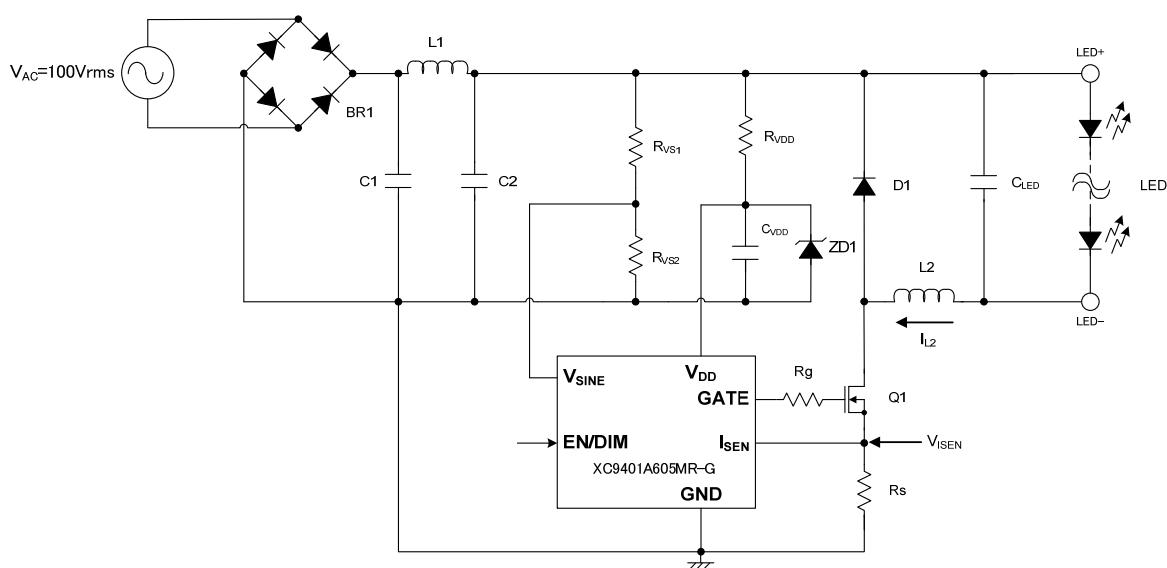
Fig.1. Reference Circuit
