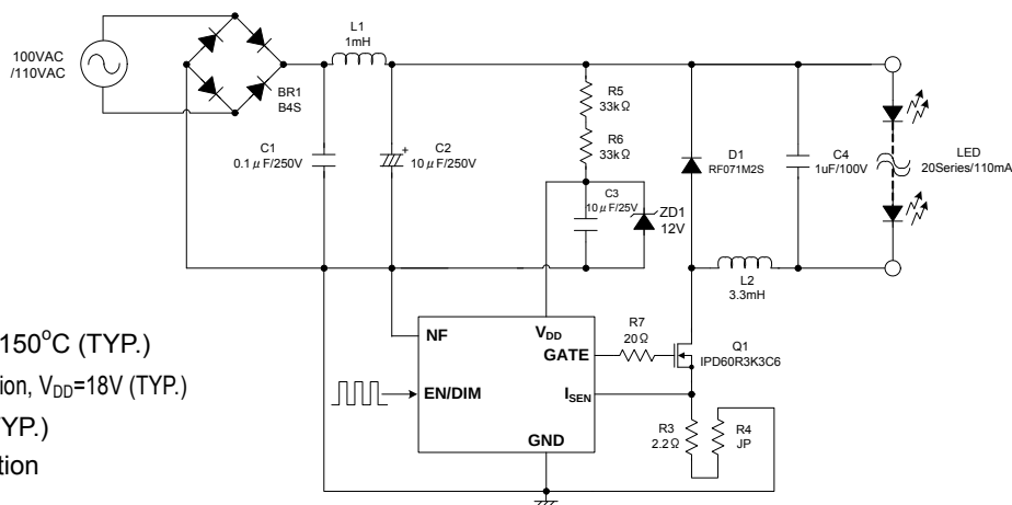
(XC9401B605MR-G 100VAC Non-isolation buck Type)
