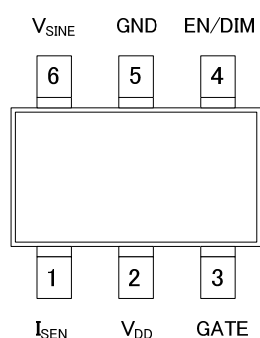
SOT-26 (TOP VIEW)
