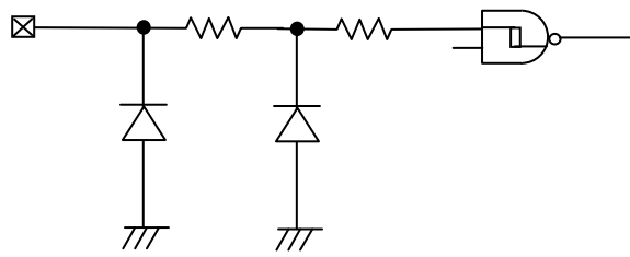
Fig.58 Input pin circuit diagram
