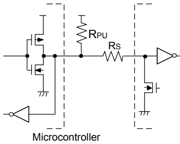
Fig.52 I/O circuit diagram
