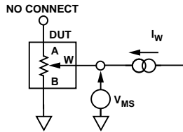
Figure 29. Potentiometer Divider Nonlinearity Error Test Circuit (INL, DNL)
