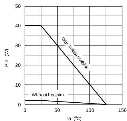
FKG1020 PD-Ta Characteristics
