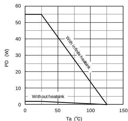
EKG1020 PD-Ta Characteristics
