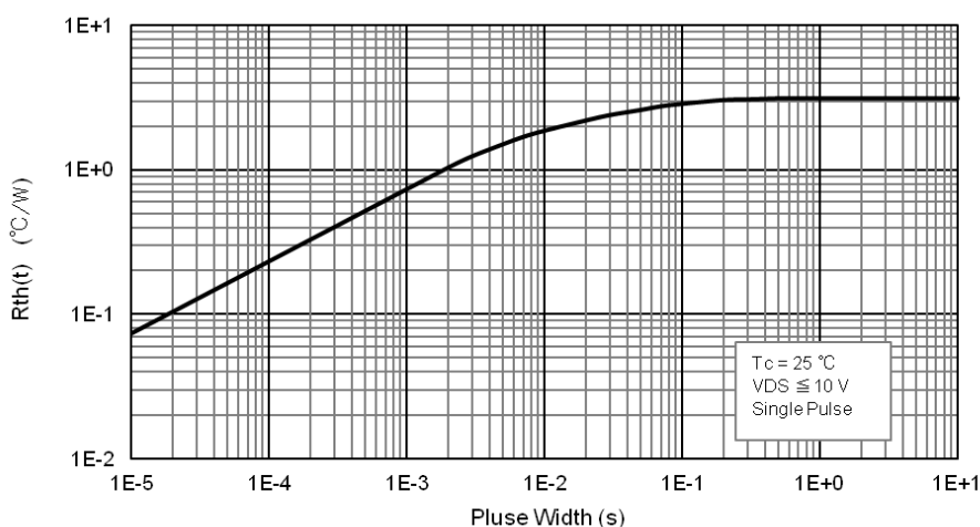
FKG1020 Transient Thermal Resistance - Pulse Width
