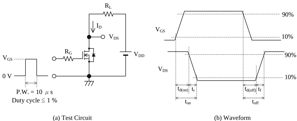
Figure 3. Switching Time
