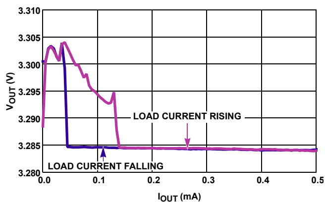
FIGURE 24. OUTPUT VOLTAGE vs LOAD CURRENT ( V_{IN} = 4.5V , V_{OUT} = 3.3V , AUTO PFM/PWM MODE)
