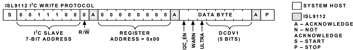
FIGURE 30. I 2 C REGISTER WRITE PROTOCOL
