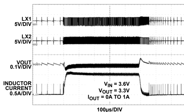
FIGURE 14. TRANSIENT LOAD RESPONSE
